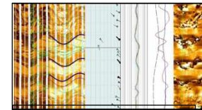
Borehole Images
