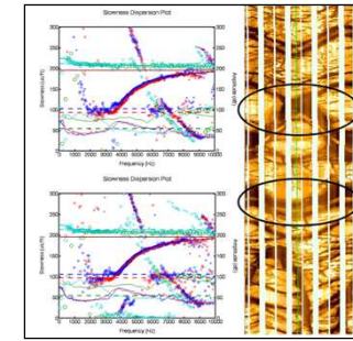
Shear Anisotropy
