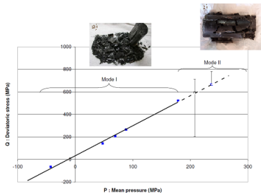
FIGURE: Brittle behavior : Failure criterion (Deviatoric stress versus Mean pressure). Rupture modes depend on confining pressure.
