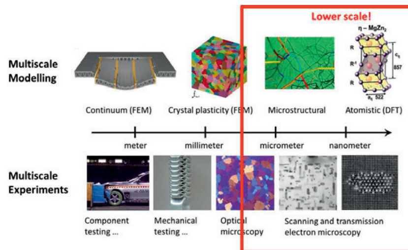
Figure 4: In a multiscale framework, the lower scale programme covers the micrometre and nanometre scales for modelling and experiments.
