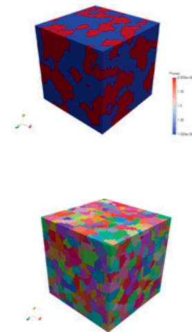
Figure 12: Example of generated microstructure.
