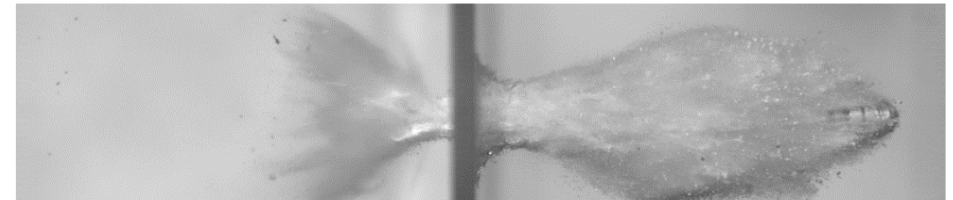
The picture above shows a test where the Phantom V1610 high-speed camera has been used. A 7 mm laminated safety glass is hit by a 7.62 calibre lead bullet at a speed of 800 m/s. The camera is set to a frame rate of 60 000 FPS and exposure time 0.452 \mu s.
