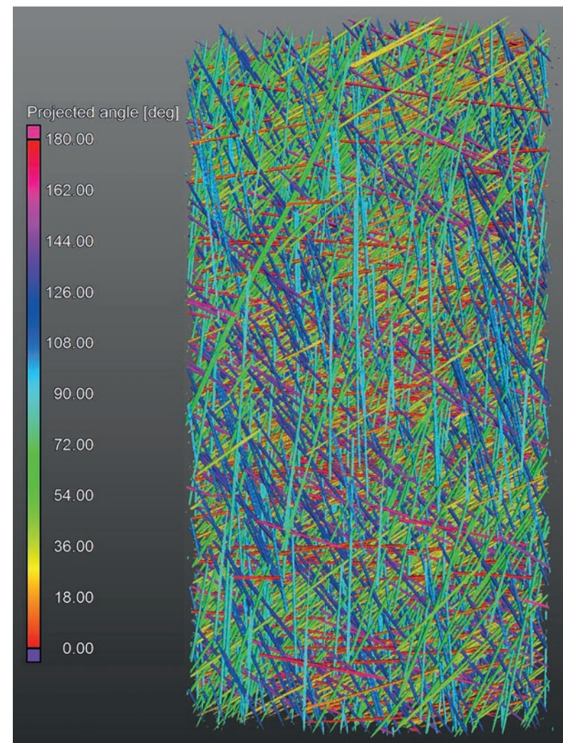
Figure 6: Computer tomography (CT) scan of glassfibre – reinforced polypropylene (PP).
