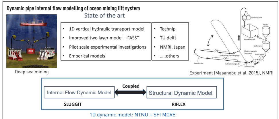
Figure 1: The coupled dynamic model concept
