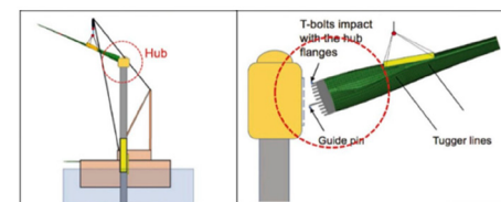
Figure 3: Blade root sideways impact and damage in guide pin and root laminate
