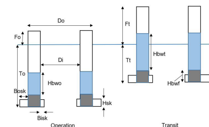
Figure 1: Illustration of the design variables of the floating dock
