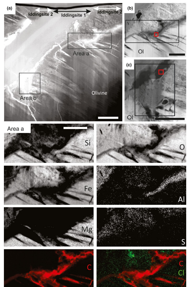
FIGURE 6 Distribution and elemental mapping of olivine (Ol), iddingsite alteration and organic carbon in Y000593. (a) BF (bright field) STEM image of FIB-lamella-3 (for location in sample see Figure 3b) the black boxes correspond to areas that were selected for element mapping. (b) High-angle annular dark field (HAADF) STEM image of Area a, contains fractured olivine (lower right) adjacent to iddingsite (upper left), element maps shown beneath. (c) HAADF STEM image of Area b on the margin of a brecciated and altered olivine crystal (lower right), elemental maps shown in Figure 7. Area a
