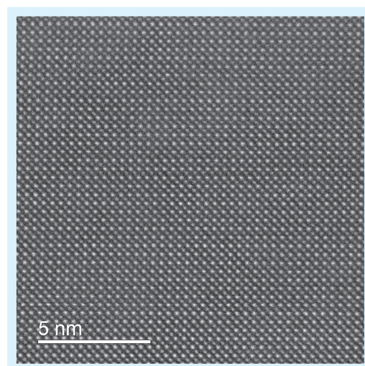
HAADF-STEM images of a SrTiO 3 /BaTiO 3 (STO/BTO) thin film. Specimen preparation by Inger-Emma Nylund. Images by Dipanwita Chatterjee.
