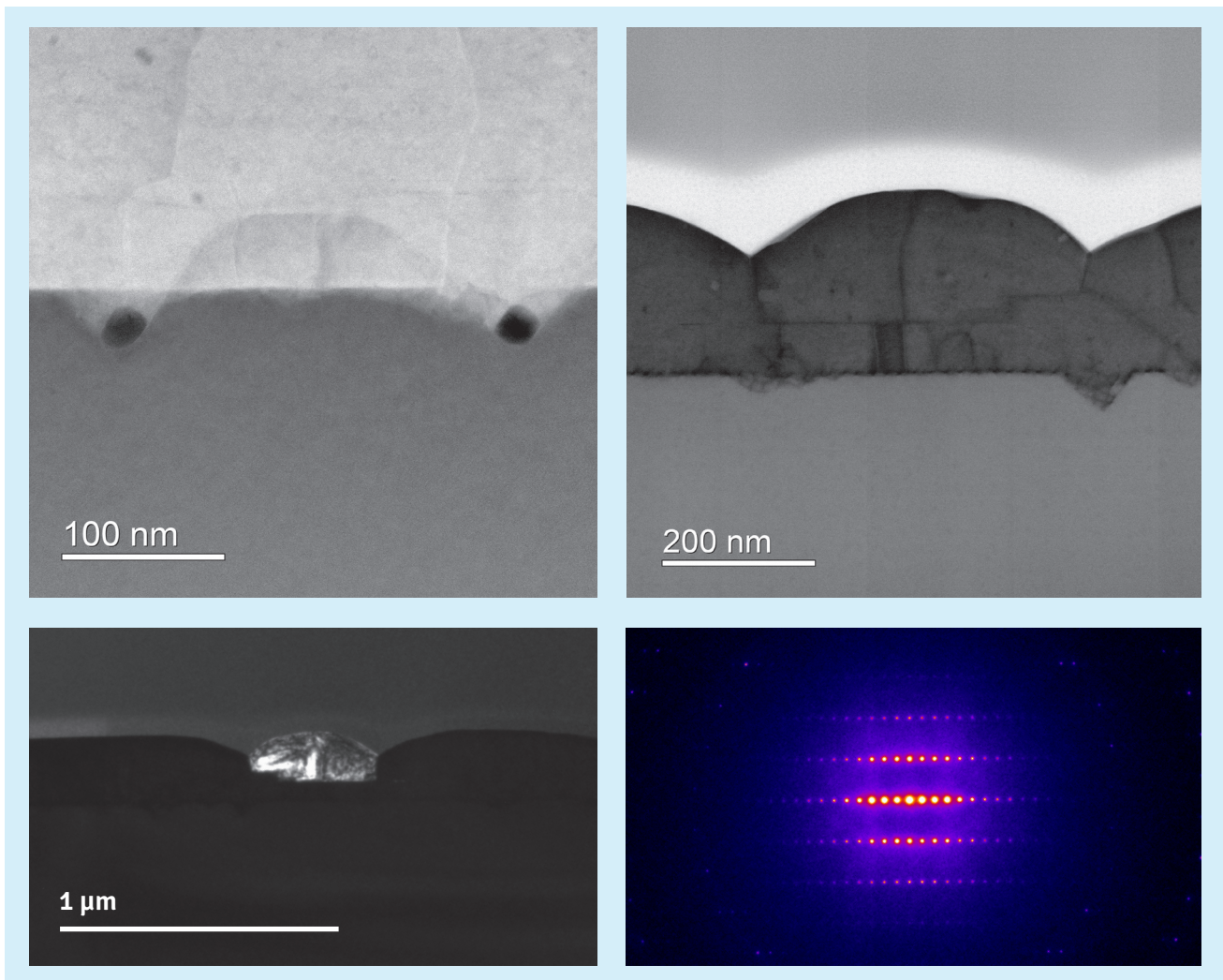
Chemical solution deposited \text{BaTiO}_3 thin film on a \text{SrTiO}_3 substrate oriented to [111] : top left; defective \text{SrTiO}_3 substrate surface, and top right and bottom left; BF-STEM and DF-TEM images of the same grain . Bottom right: SAED pattern of \text{Gd}_2(\text{MoO}_4)_3 . By Inger-Emma Nylund.
