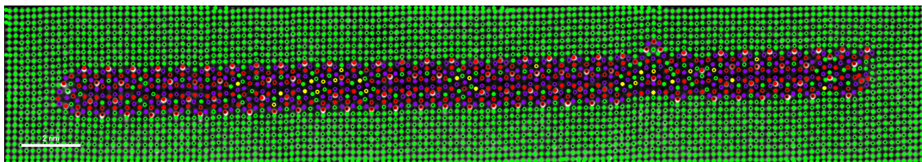
The software project AutomAI 6000 on statistical analysis and automatic atomic overlay of HAADF-STEM lattice images of precipitates in 6xxx Al alloys. Top: an 'atomic graph' that visualizes the underlying data structure of the software. Middle: the graphical user interface of the software. Bottom: a HAADF-STEM image of a large C-plate precipitate in an Al matrix overlaid by the software. By Haakon Tvedt.
