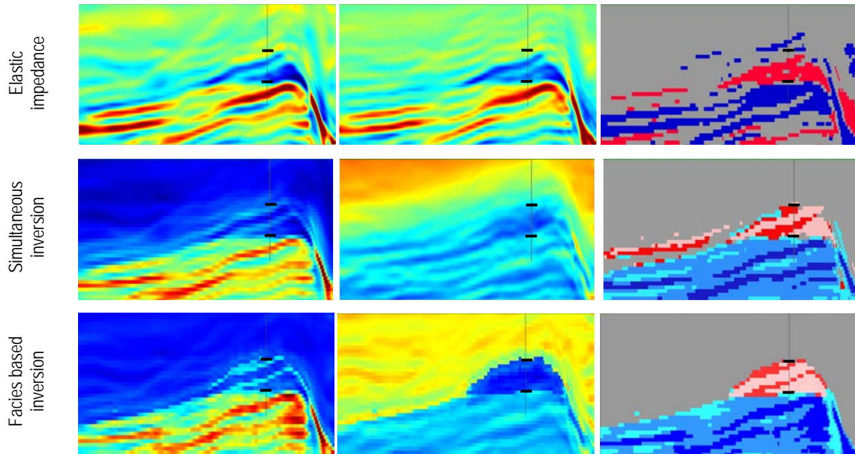
Figure 1: Inversion results and interpretation of a carbonate reef: elastic impedance inversion of near and far stack plus interpretation (top row); standard simultaneous inversion AI, V_p/V_s and interpretation (middle row); facies based inversion AI, V_p/V_s and facies (bottom row). Interpretations show grey for shale red for gas carbonate and blue for brine carbonate. Darker colours represent lower porosity for the carbonates where available.
