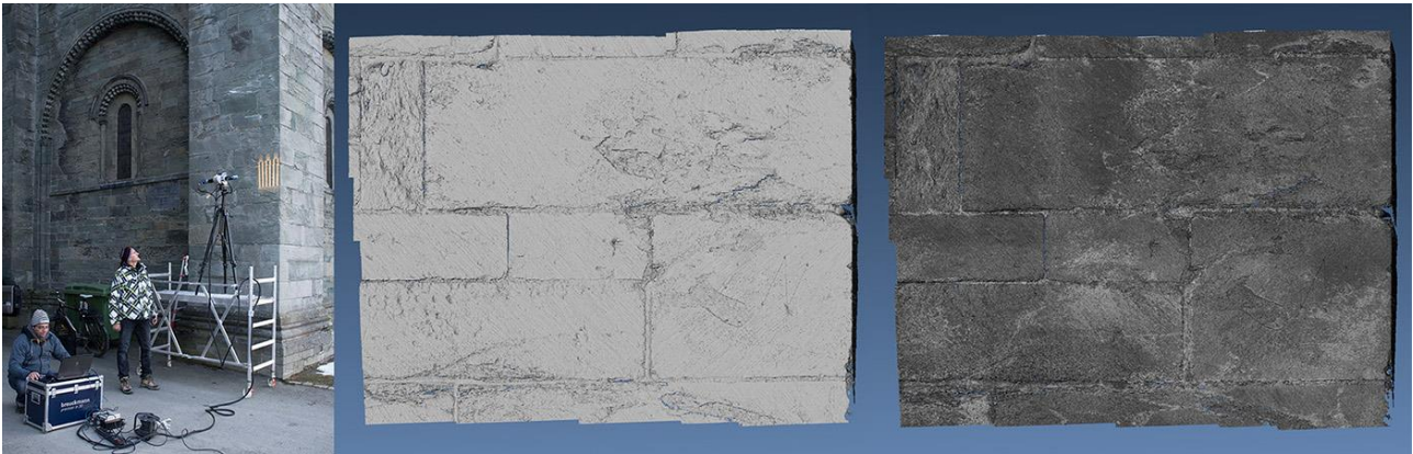
Fig. 9 - Scanning outside of the north entrance of Nidaros cathedral (left). The result from monochrome texture mapping (right) using sensor imagery provides an added value for documentation and visualisation. The scanned areas span approximately 1 by 0.9 m 2 and show stones affected by erosion. The average resolution in x, y is approximately 0.1 mm with a z-resolution around 0.007 mm. Please also note the two mason marks engraved in the rocks (middle). Such details are hardly visible in the textured image.
