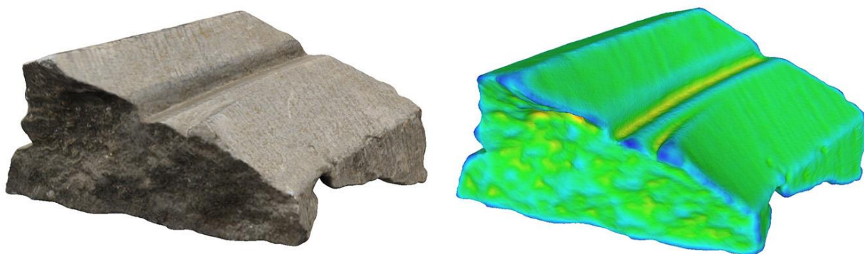
Fig. 4 - Geometry processing (curvature extraction using fast, custom descriptors) on a scanned fragment. Medium resolution models (shown here) result in comparable feature detection accuracy compared to the high resolution ones, at approx. 1/60 the computational cost.
