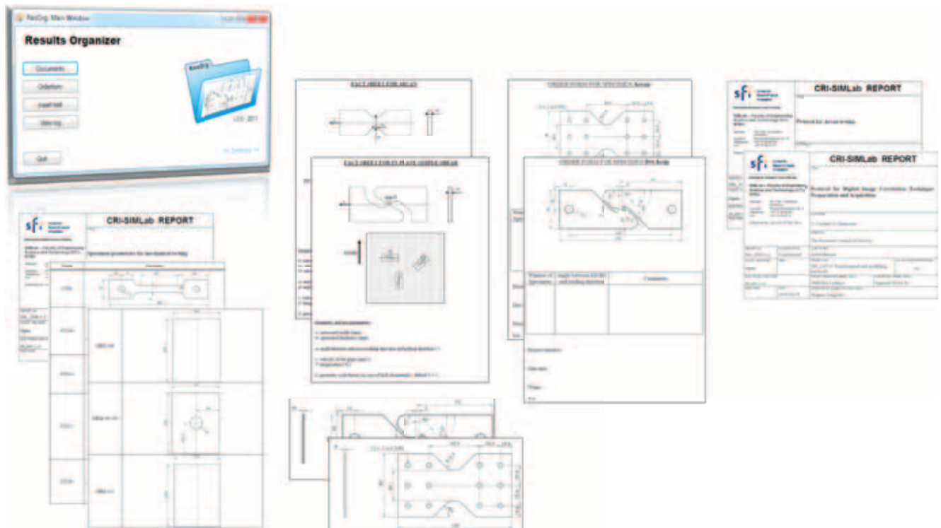
Figure 8 – ResOrg software.
