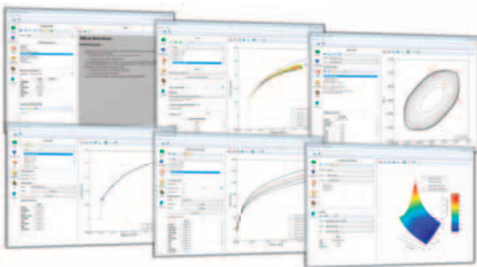
Figure 10 – MatPrePost GUI.
