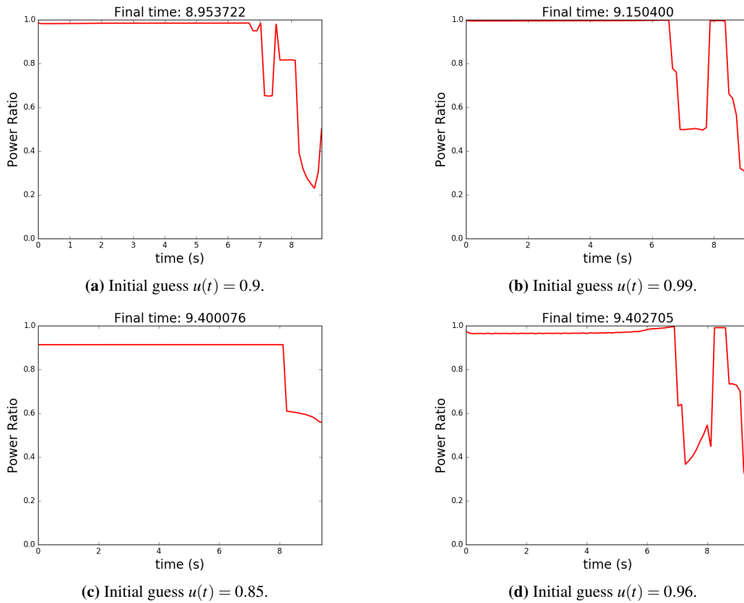
Figure 1.8: Local minima obtained with constant initial guesses.
