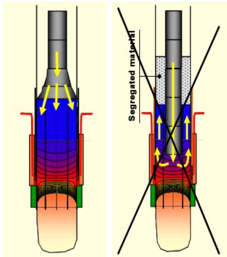
Figure 4.3: Sketches of Söderberg electrodes, illustrating the difference between a properly operating electrode (left side), and an electrode afflicted by segregation (right side).
