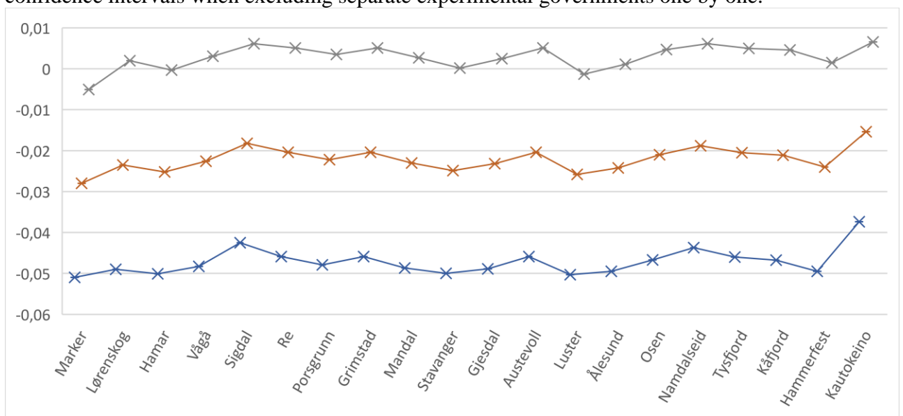
Figure 2. Estimated treatment effects and corresponding upper and lower bounds of 95% confidence intervals when excluding separate experimental governments one by one.
