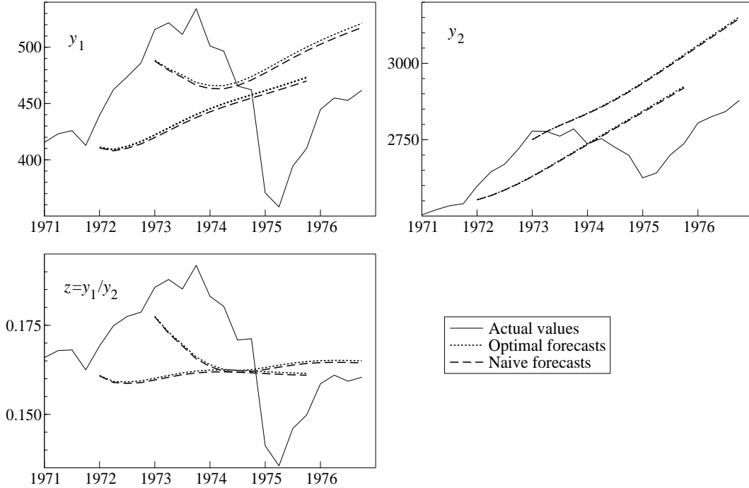
Figure 6: Dynamic forecasts for 16 periods of real investment y_1 , real GNP y_2 , and their ratio z = y_1/y_2 , starting in 1972(1) and 1973(1).
