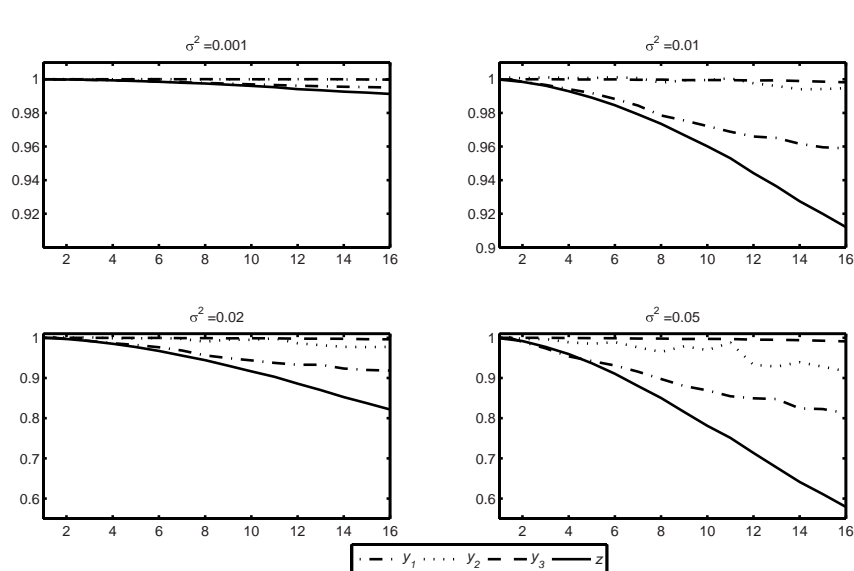
Figure 1: RMSEs of true optimal relative to estimated optimal h -step forecasts for y_t and z_t = y_{1t}/y_{2t} with deterministic terms \nu_i = 0.02 and cointegration adjustment \alpha_{11} = 0.1 , varying the covariance matrix of the residuals.
