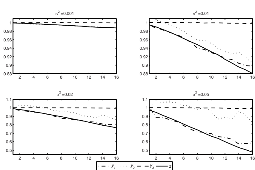
Figure 3: RMSEs of estimated naive relative to estimated optimal h -step forecasts for y_t and z_t = y_{1t}/y_{2t} with \nu_i = 0.02 and cointegration adjustment of \alpha_{11} = 0.1 , varying the covariance matrix of the residuals.
