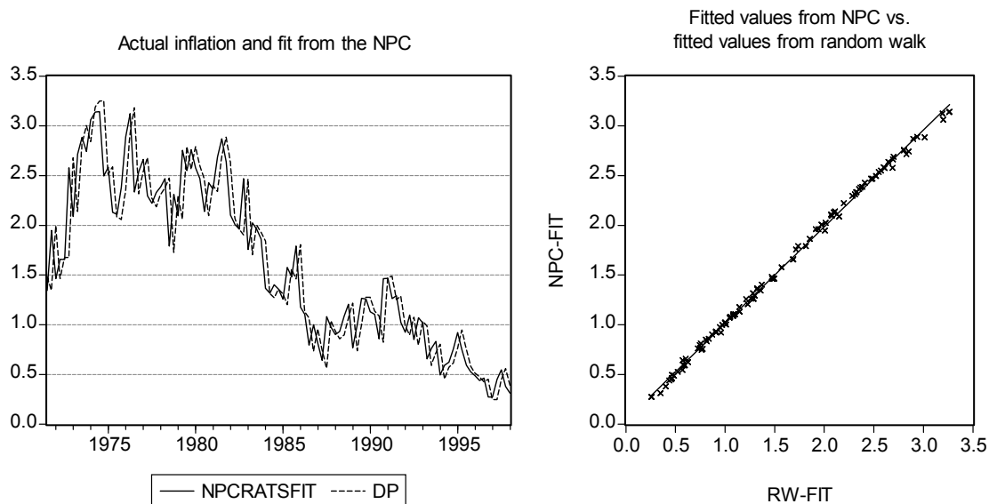
Figure 3: Actual and fitted values of equation (13) together with the fit of a random walk.
