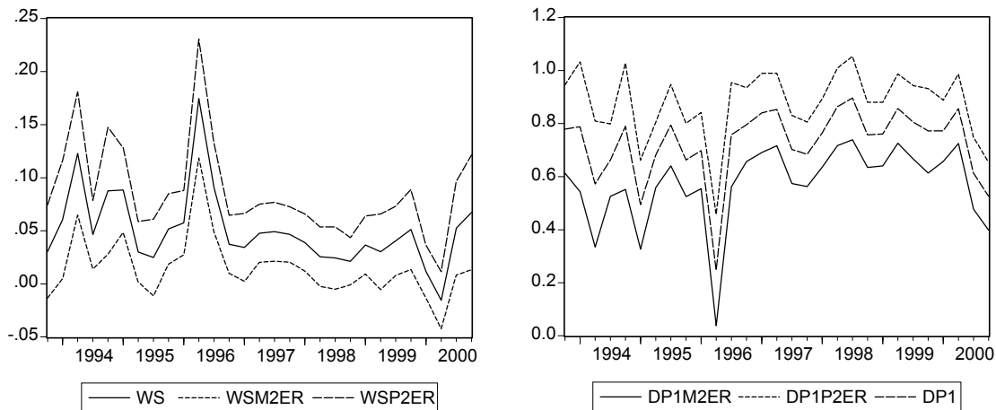
Figure 4: Rolling regression coefficients \pm 2 standard errors of the New Keynesian Phillips curve, estimated on Norwegian data ending in 1993.4 - 2000.4.
