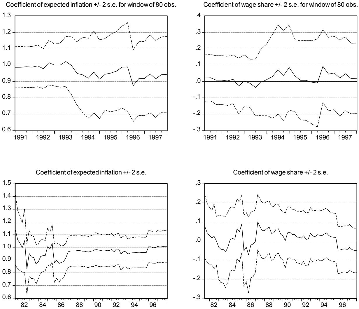
Figure 2: The upper graphs show rolling regression coefficients \pm 2 standard errors of the New Keynesian Phillips curve for the Euro area equation (14), i.e., estimated with GMM. The lower graphs show the recursive estimates of those coefficients.
