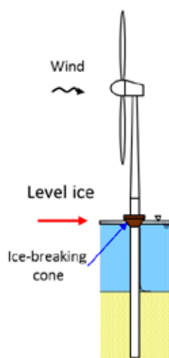
Figure 40: Monopile wind turbine with ice-breaking cone.
