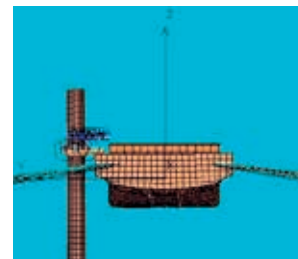
Figure 24: Dynamic coupled model of vessel and MP during initial hammering process.
