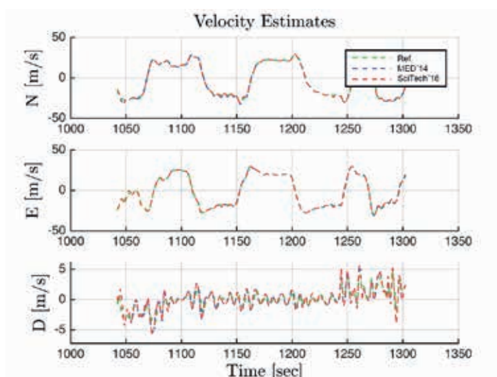
Figure 11: North-East-Down velocity estimates for the two nonlinear observers (flat terrain).
