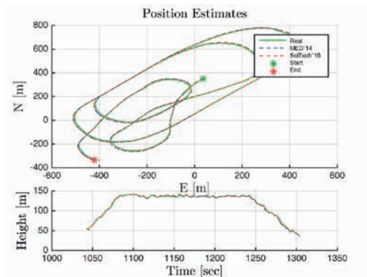
Figure 10: North-East-Down position estimates for the two nonlinear observers (flat terrain).
