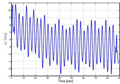
(f) Joint angle offset, \phi_0
