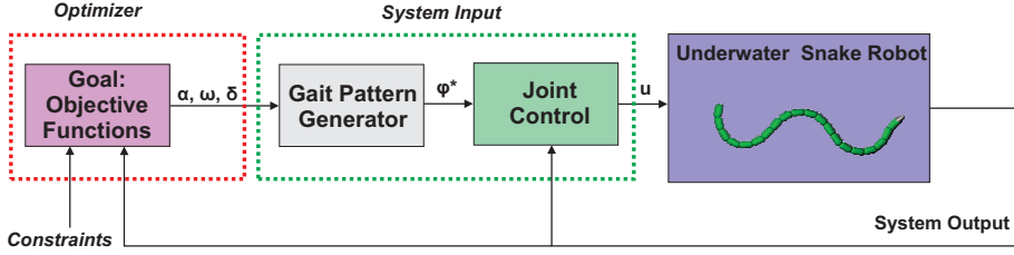
Figure 7.22: Illustration of the optimization framework.
