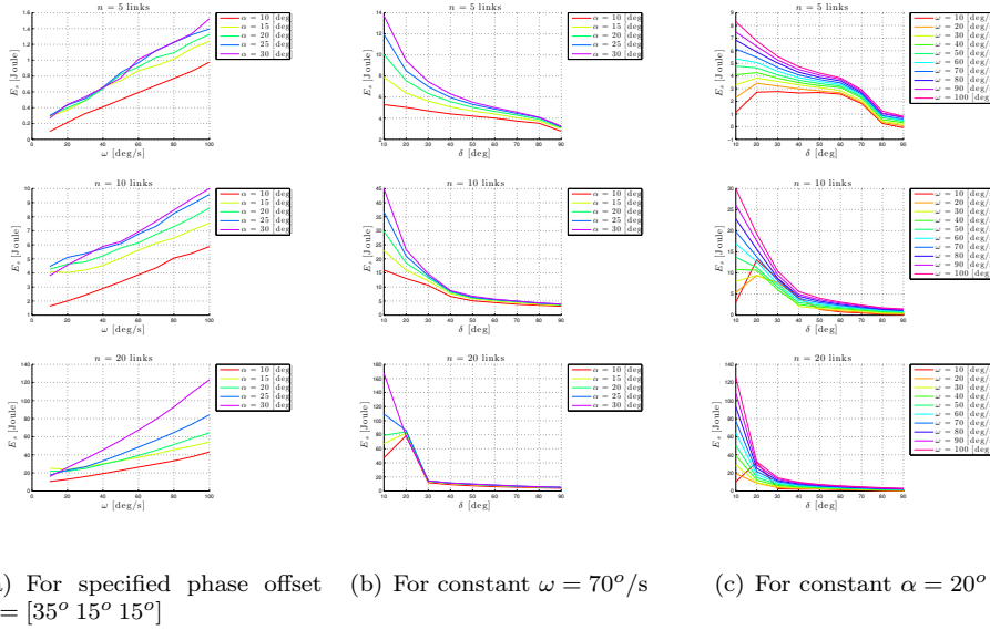
Figure 7.18: Total energy consumption for the eel-like motion pattern.
