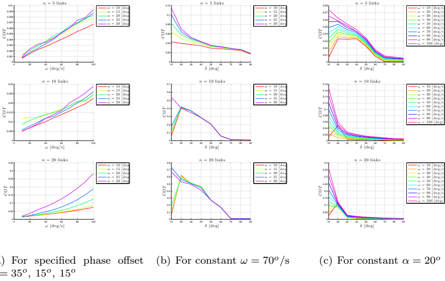
Figure 7.17: Cost of transportation for the lateral undulation motion pattern.
