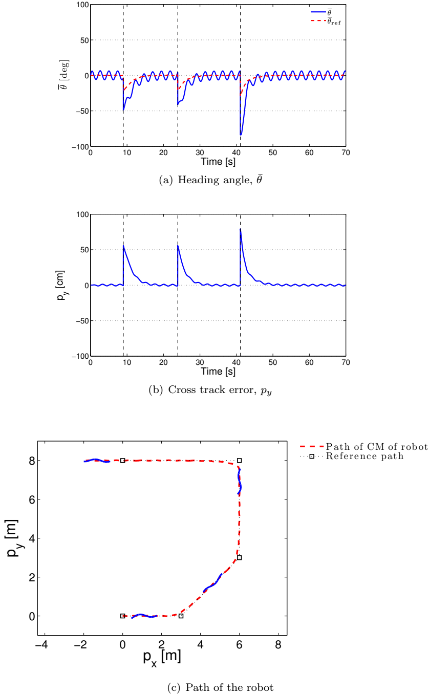
Figure 6.34: Path following of underwater snake robot during waypoint guidance for lateral undulation.
