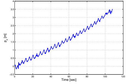
(b) Position along the path, p_x
