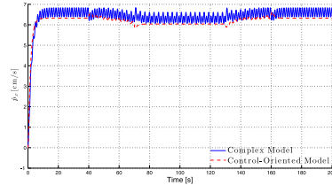
(b) CM velocity in x direction, \dot{p}_x
