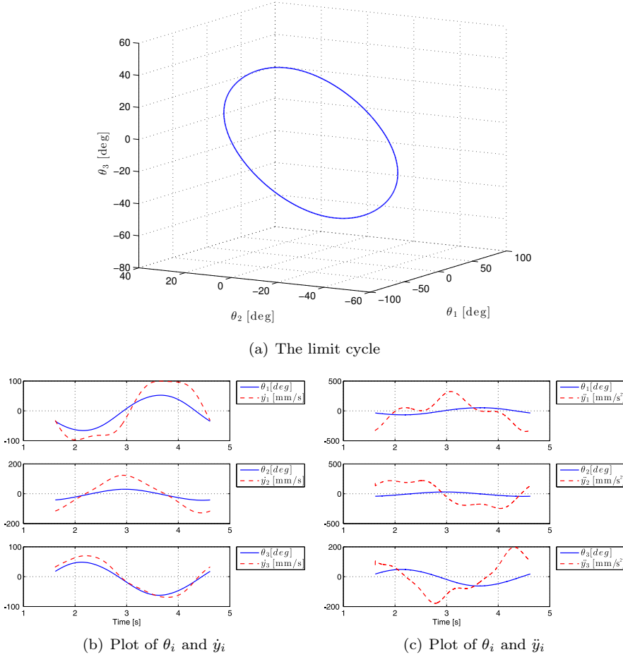
Figure 6.9: Stability analysis of the Poincaré map for lateral undulation.
