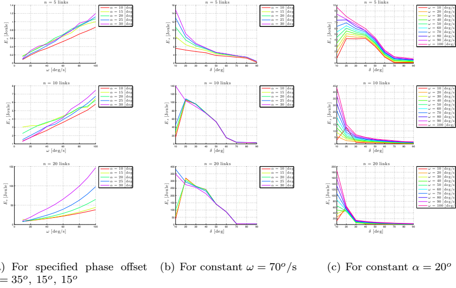
Figure 7.16: Total energy consumption for the lateral undulation motion pattern.
