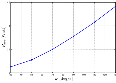
(c) Simulations: \alpha = 30^\circ and \delta = 30^\circ
