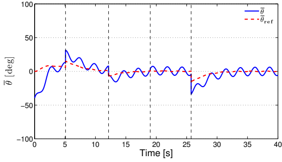
(a) Heading angle, \bar{\theta}
