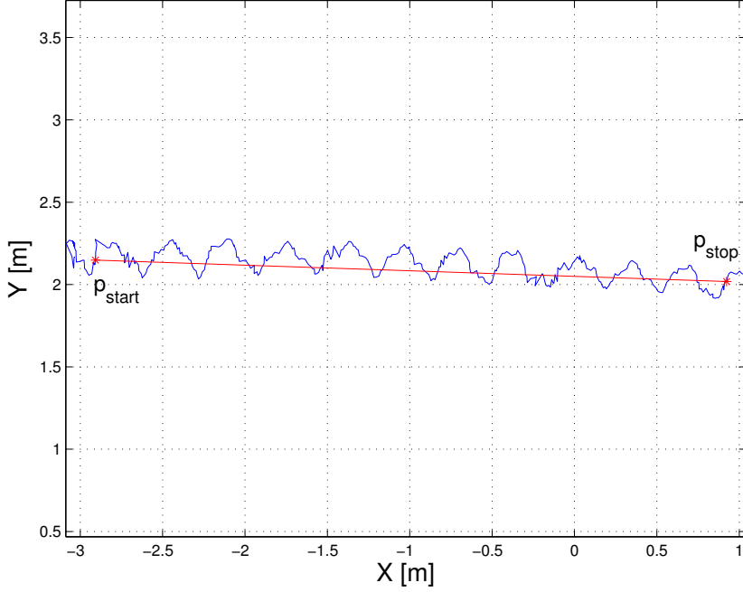
Figure 5.18: Measured position of the underwater snake robot during eel-like motion pattern. The distanced travelled by the robot is shown with red color.
