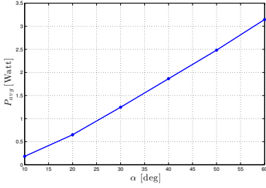
(a) Simulations: \omega = 120^\circ/\text{s} and \delta = 30^\circ
