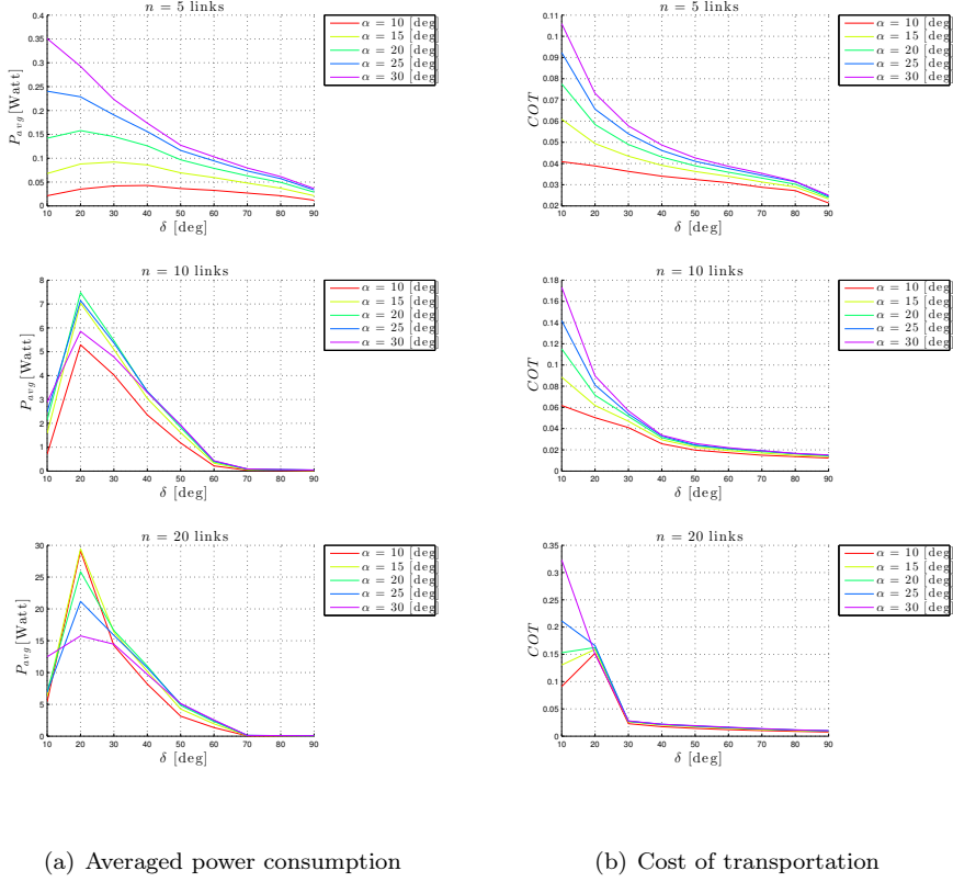
Figure 7.6: Simulation results for the lateral undulation motion pattern with constant frequency \omega = 70^\circ/\text{s} .
