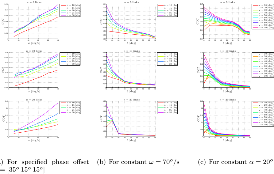
Figure 7.19: Cost of Transportation for the eel-like motion pattern.
