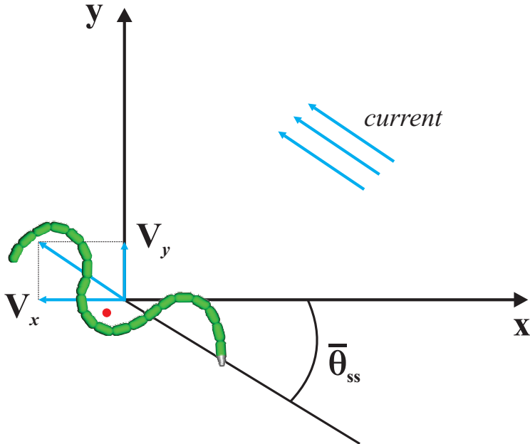
Figure 6.6: Steady state: The underwater snake robot side-slips with a constant \bar{\theta}_{ss} to follow the path.
