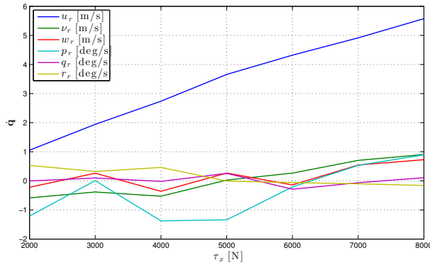
Figure 7.13: Simulation results for the velocities of the ROV.
