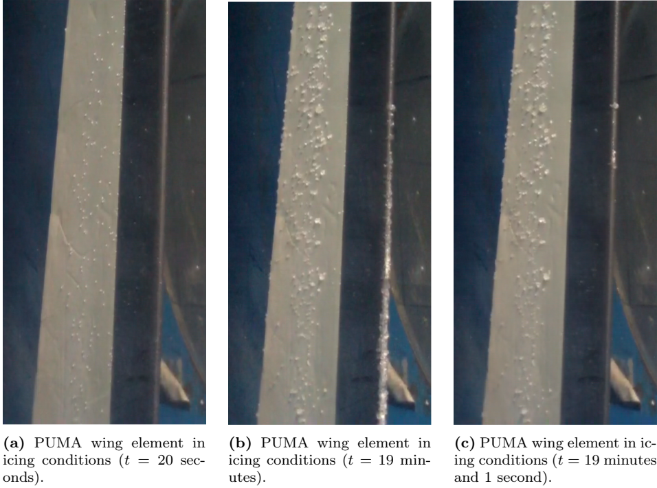
Figure 9.13: PUMA platform wing element in De-Icing experiment, conducted in icing conditions.
