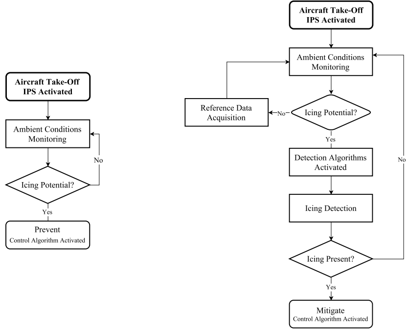
Figure 6.3: High level IPS operational flow-chart for two of the three control algorithm procedures.
