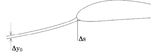
Figure 2.14: Definition of collection efficiency [2].
