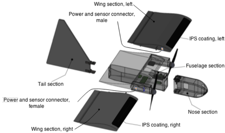
Figure 8.2: Diagram of Dragon Eye UAV platform, including detachable components and IPS integration.
